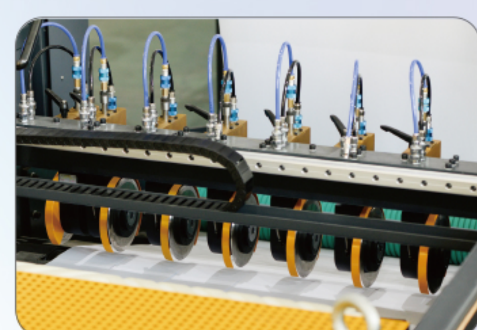
分条刀 Slitting knife
