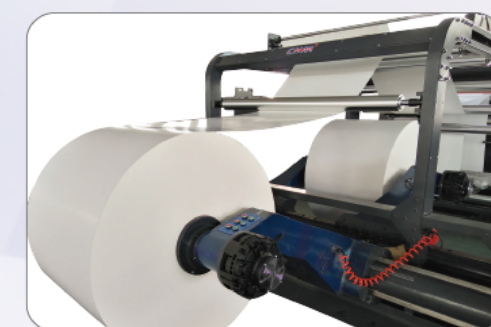
双臂液压无轴原纸架 Hydraulic shaft-less unwind station
