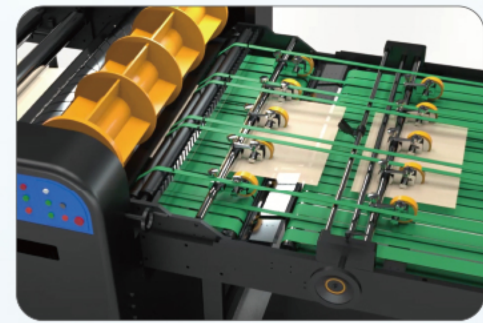
高精度单刀切纸机 High precision single rotary sheet cutter
